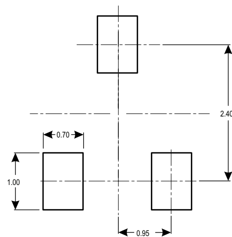
B PCB Layout Reference View
