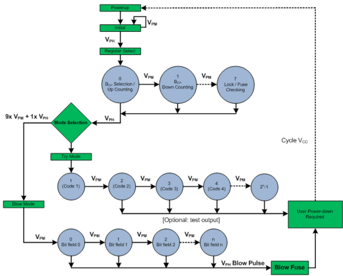
Figure 10. Programming state diagram
