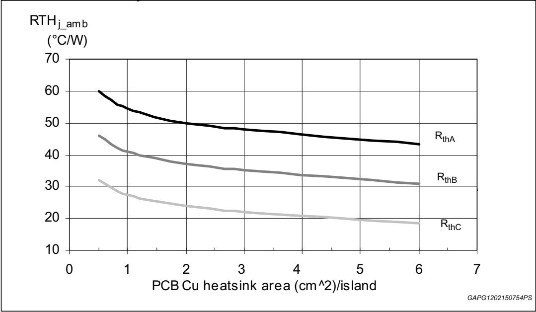
Figure 23. R_{thj-amb} Vs PCB copper area in open box free air condition
