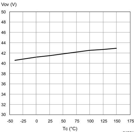
Figure 14. Overvoltage shutdown
