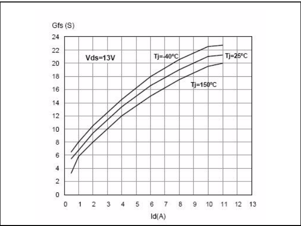
Figure 13. Transconductance
