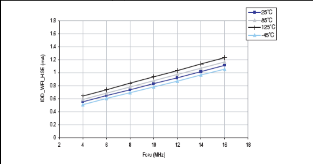
Figure 16. Typ I_{DD(WFI)} vs. f_{CPU} HSE external clock, V_{DD} = 5\text{ V}
