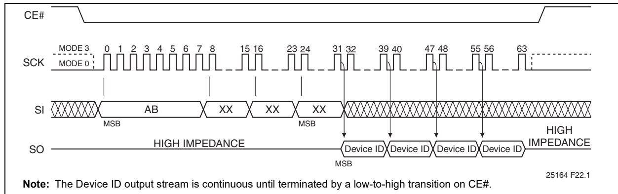
FIGURE 5-15: READ-ID SEQUENCE
