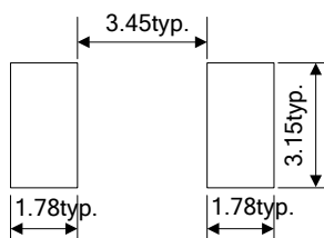
Recommended Pad Layout (mm)
