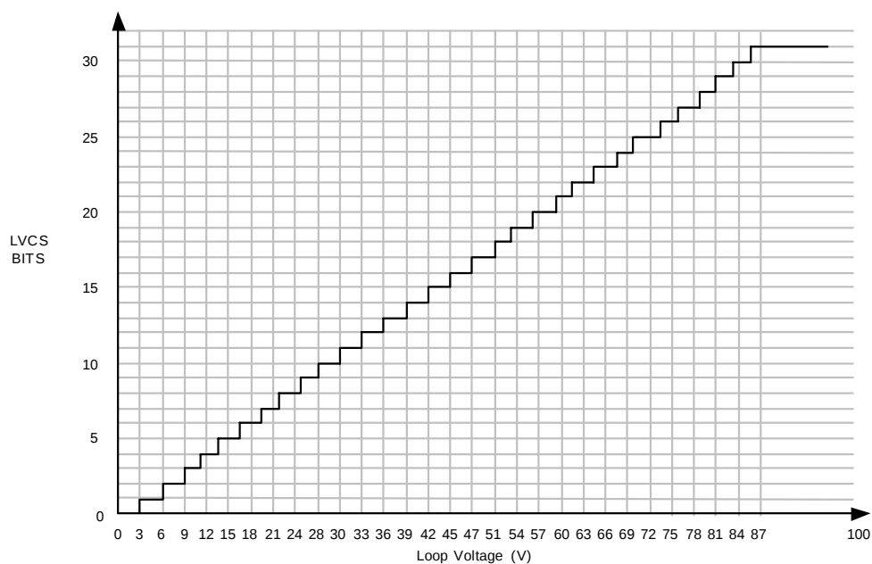
Figure 6. Loop Voltage
