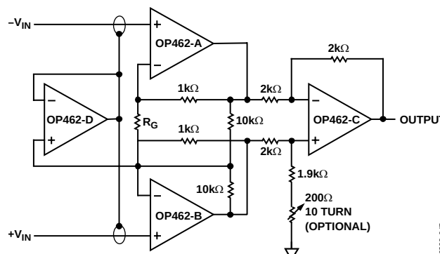
Figure 44. High Speed Instrumentation Amplifier
