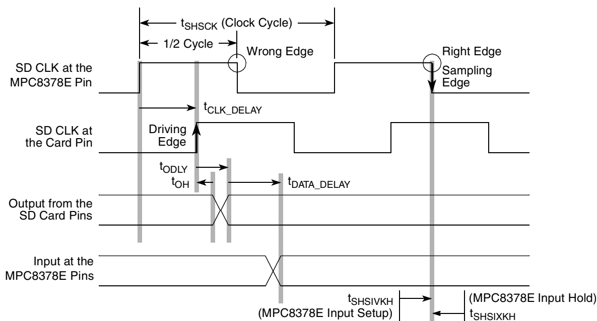
Figure 35. High-Speed Input Path
