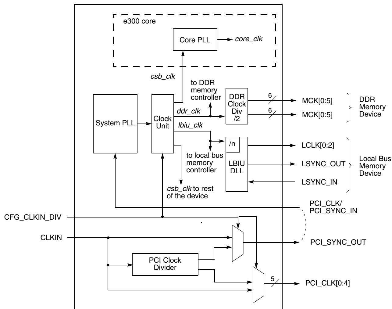
Figure 64. Clock Subsystem
