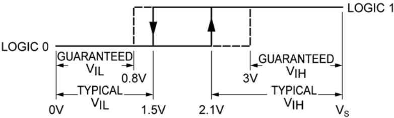
Figure 3. Input Hysteresis
