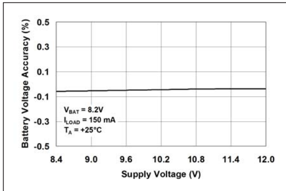
FIGURE 2-13: Battery Voltage Accuracy ( V_{RTO} ) vs. Supply Voltage ( V_{DD} ).
