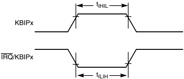
Figure 14. \overline{\text{IRQ}}/\text{KBIPx} Timing
