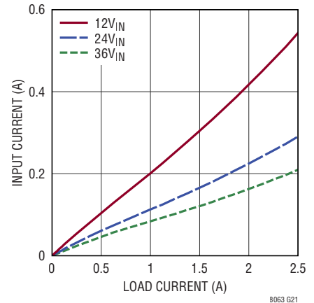
Input vs Load Current V_{OUT} = 2V
