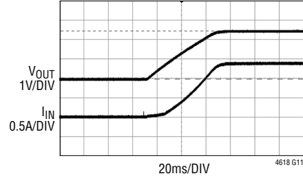
Start-Up, I_{OUT} = 6A
