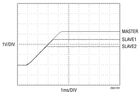
Figure 1. Coincident Tracking
