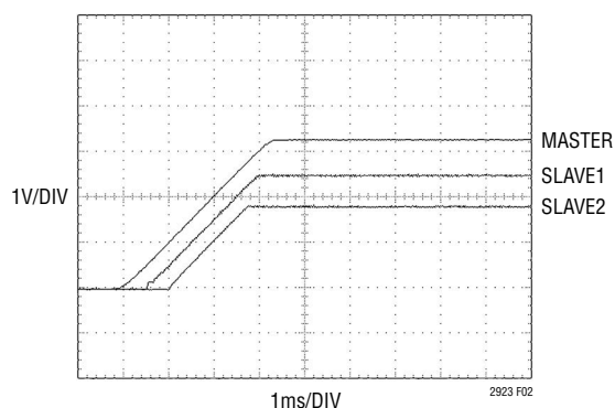
Figure 2. Offset Tracking
