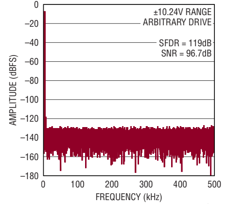
32k Point Arbitrary Two-Tone FFT f_{SMPL} = 1\text{Mps} , IN^+ = -7\text{dBFS} 2kHz Sine, IN^- = -7\text{dBFS} 3.1kHz Sine
