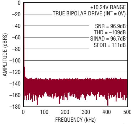
32k Point FFT f_{SMPL} = 1\text{Mps} , f_{IN} = 2\text{kHz}
