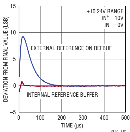
Figure 12. Burst Conversion Response of the LTC2335-18, f_{\text{SMPL}} = 1\text{Mps}
