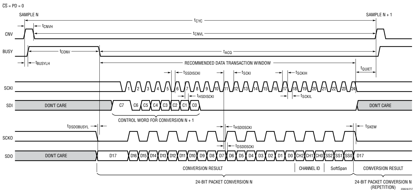
Figure 17. Serial CMOS I/O Mode, Direct Per-Conversion Configuration
