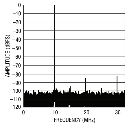
LTC2265-14: 8k Point FFT, f_{IN} = 140\text{MHz} , -1dBFS, 65Mps
