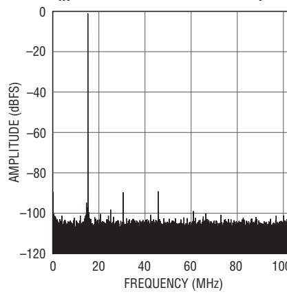
LTC2156-12: 32K Point FFT, f_{IN} = 15\text{MHz} , -1dBFS, 210Msps
