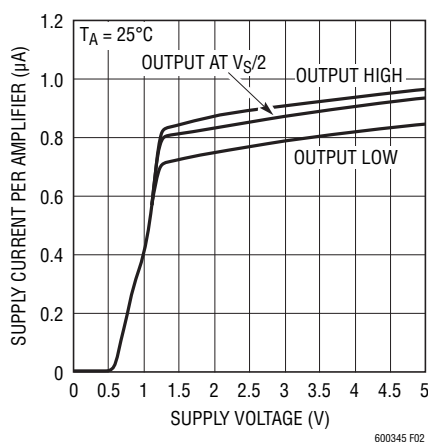
Figure 2. Start-Up Characteristics
