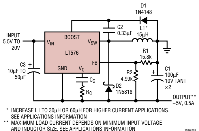
Figure 15. Positive-to-Negative Converter
