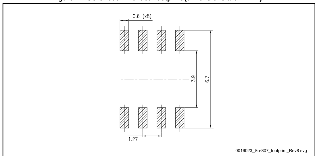
Figure 14: SO-8 recommended footprint (dimensions are in mm)
