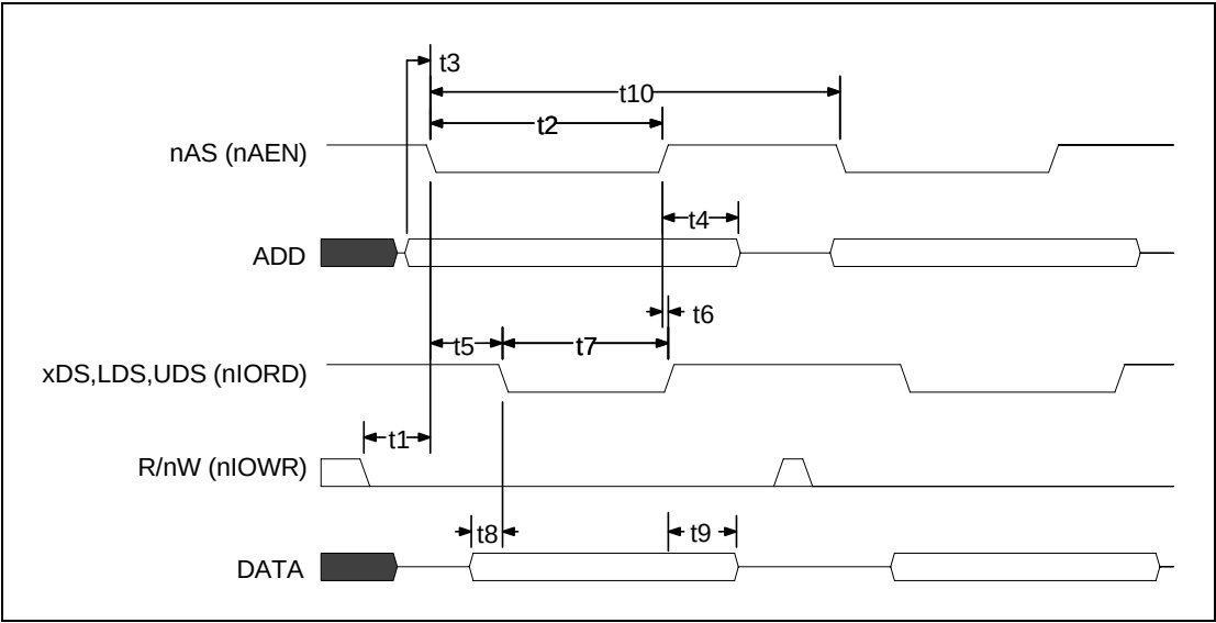
Figure 12.11 - 68000 Write Timing
