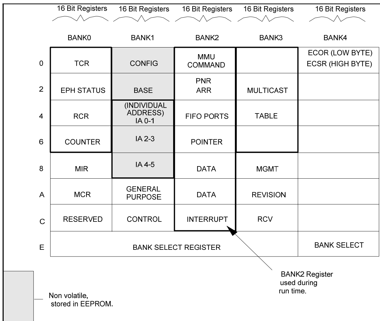
Figure 6.2 - LAN91C96 Registers
