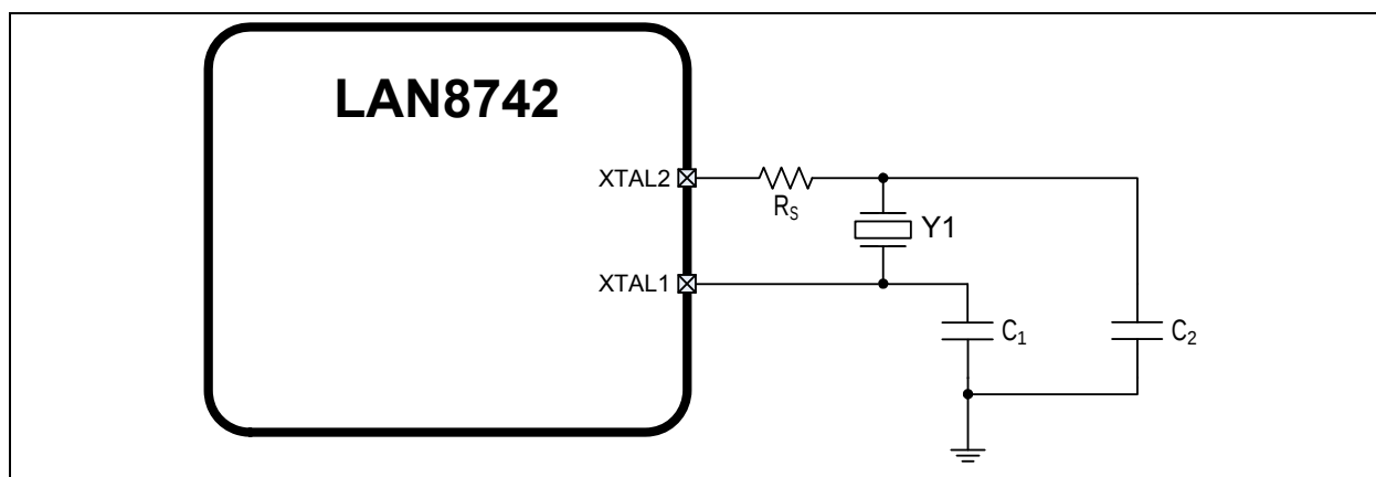
FIGURE 5-8: 100 \mu\text{W} 25 MHZ CRYSTAL CIRCUIT
