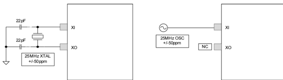
Figure 6. 25MHz Crystal / Oscillator Reference Clock
