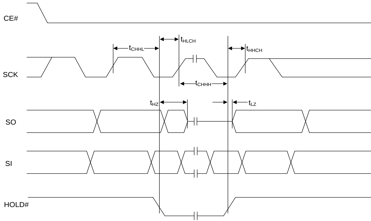
Figure 9.4 HOLD TIMING
