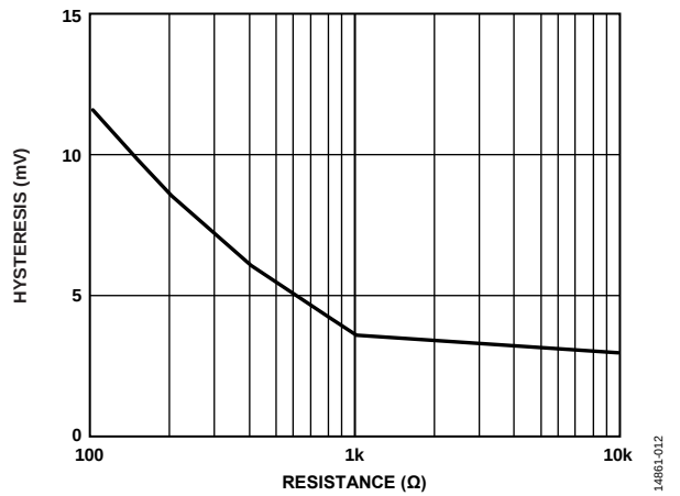
Figure 12. Comparator Hysteresis vs. R_{HYS} Control Resistance
