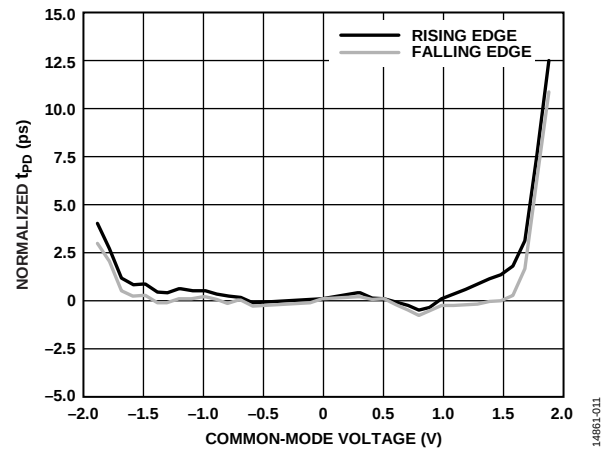
Figure 11. Normalized Propagation Delay ( t_{PD} ) vs. Common-Mode Voltage
