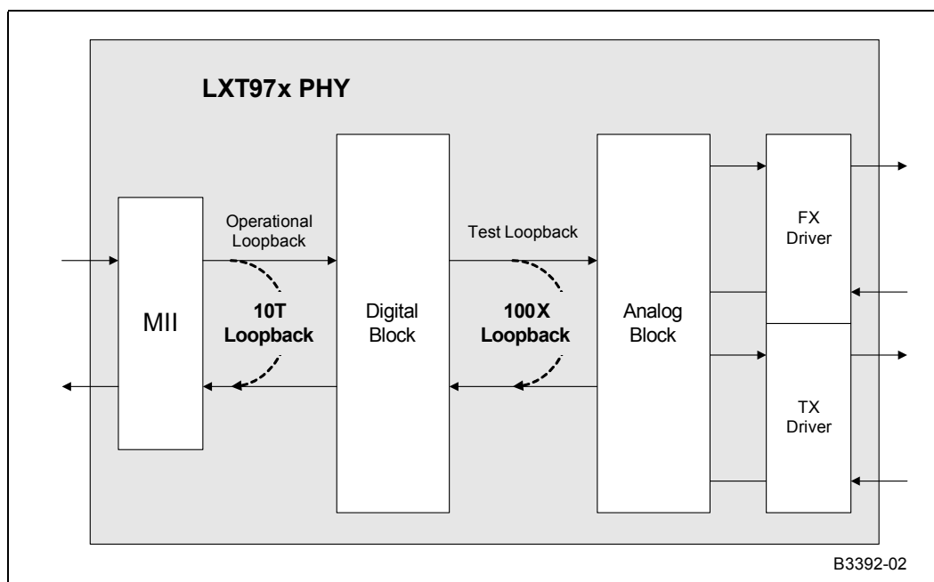
Figure 13 Loopback Paths
