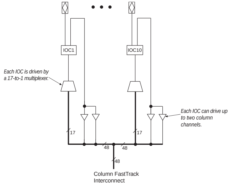
Figure 9. MAX 9000 Column-to-I/O Connections
