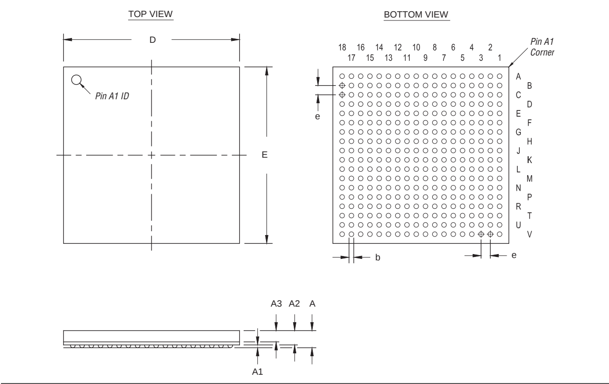
Figure 7-9. 324-Pin FineLine BGA Package Outline
