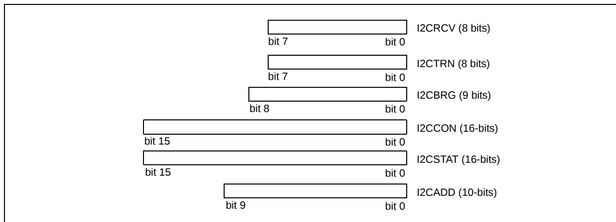
FIGURE 17-1: PROGRAMMER'S MODEL
