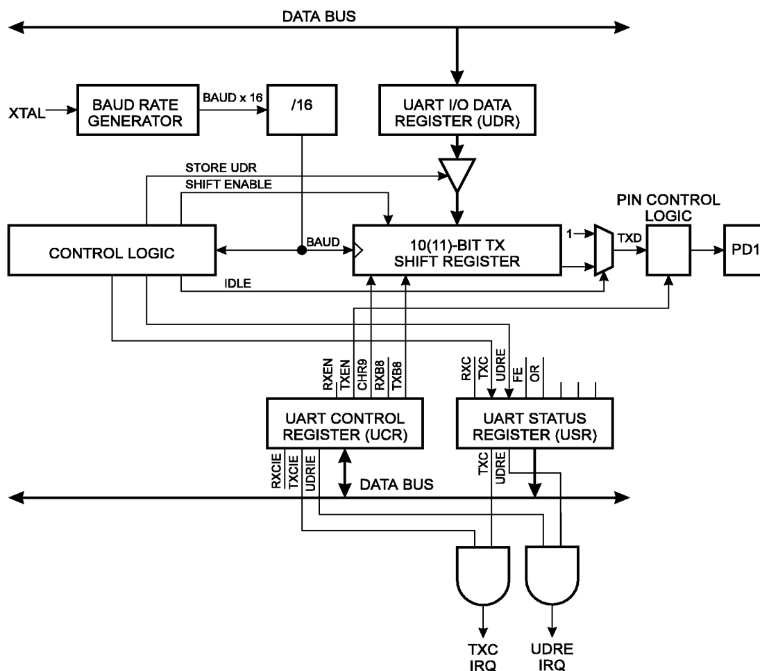
Figure 38. UART Transmitter
