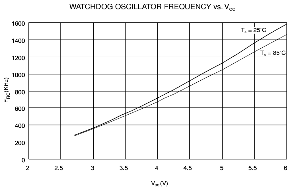
Figure 79. Watchdog Oscillator Frequency vs. V_{CC}
