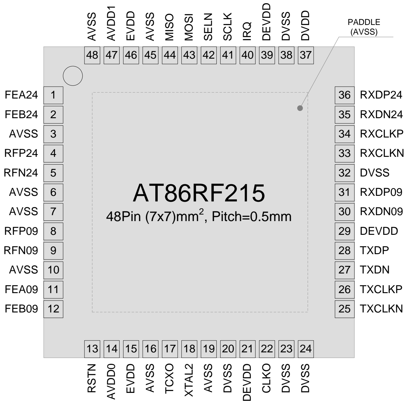
Figure 2-1. Pin-out
