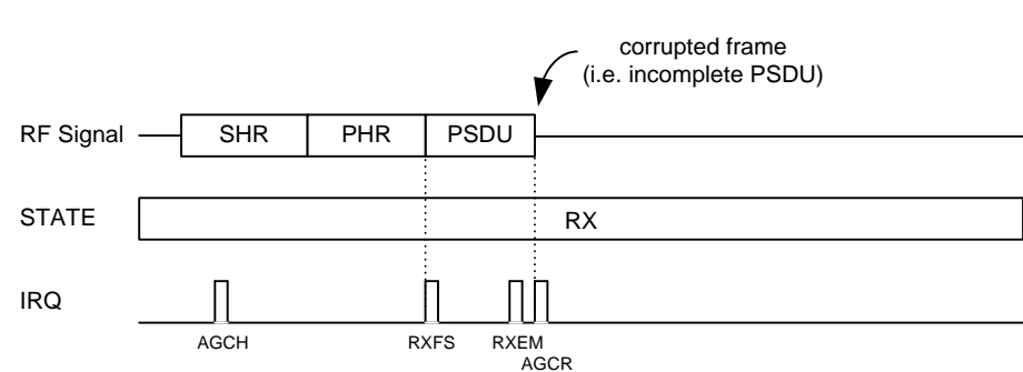
Figure 6-17. Baseband Interrupts during Canceled Frame Reception
