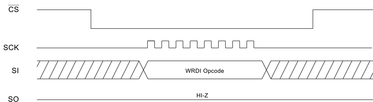
Figure 7-3. WRDI Timing
