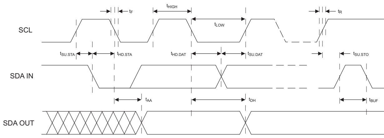
Figure 8-1. Bus Timing
