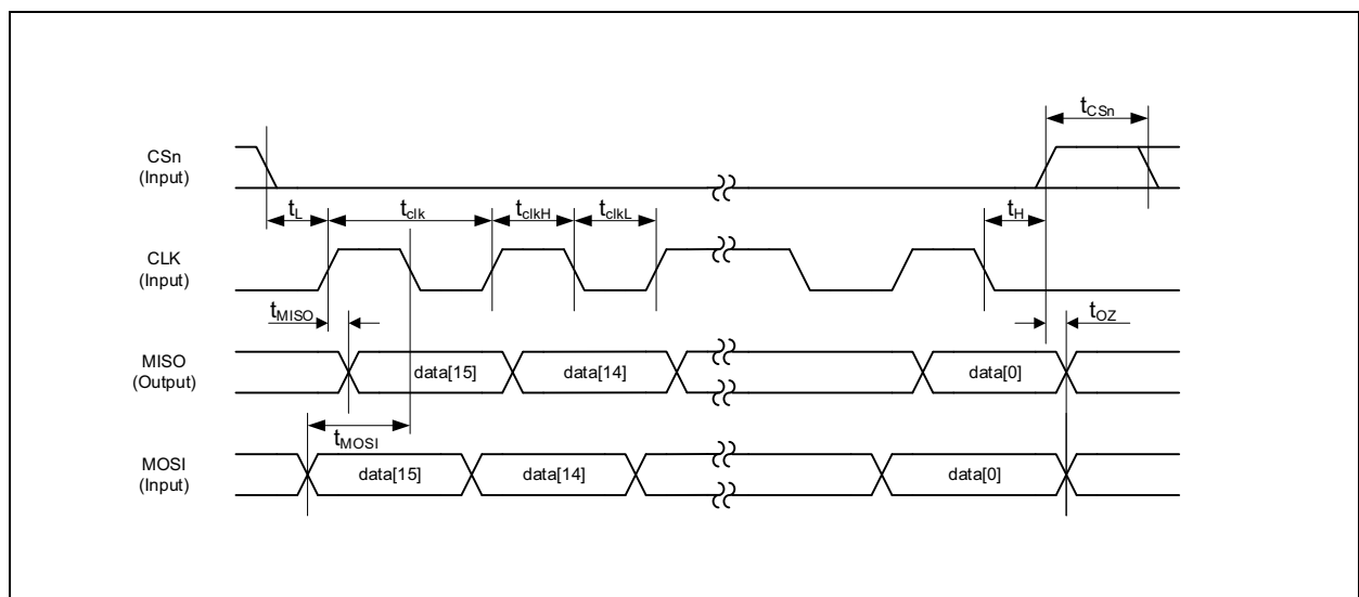
Figure 12: SPI Timing Diagram
