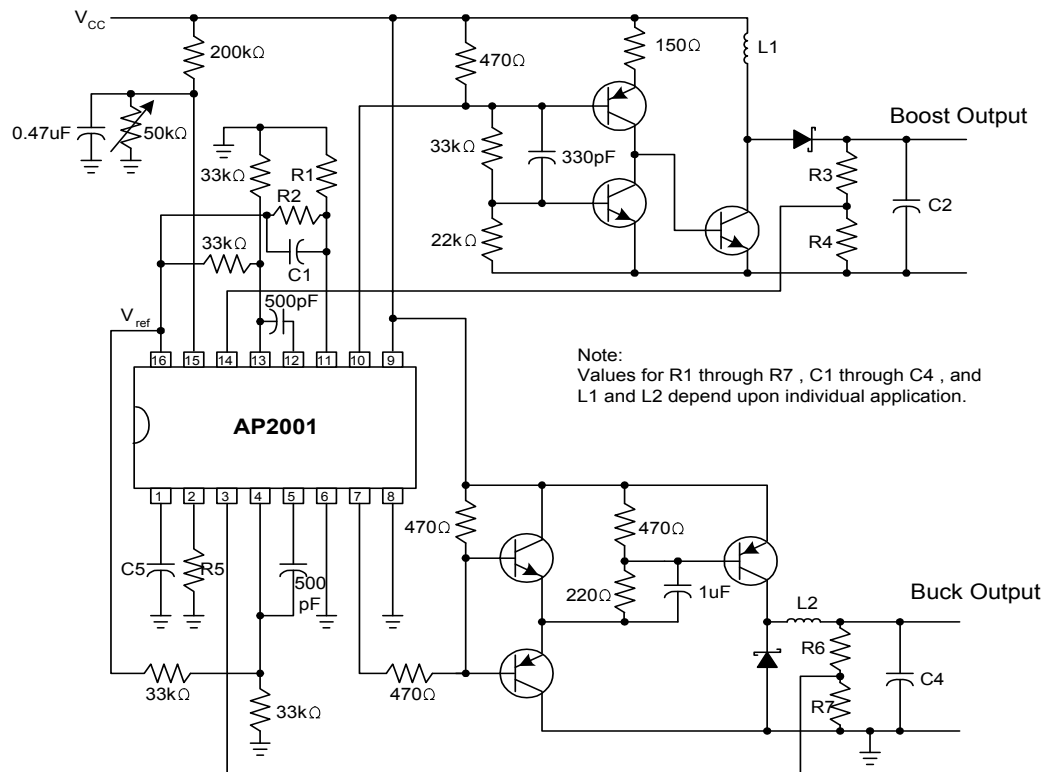
Dual output DC/DC converter
