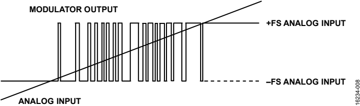
Figure 26. Analog Input vs. Modulator Output
