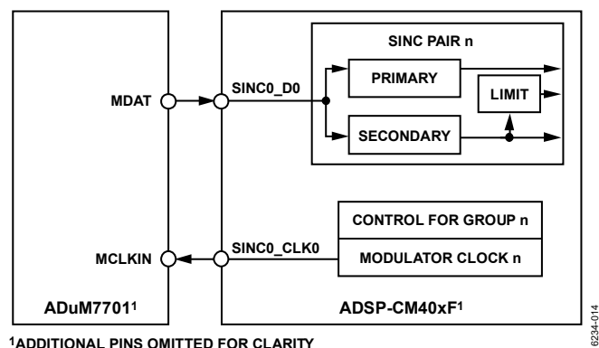
Figure 32. Interfacing the ADuM7701 to the ADSP-CM4xx
