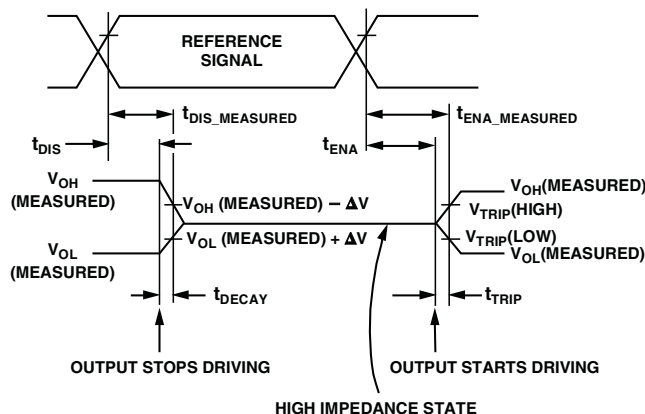
Figure 59. Output Enable/Disable
