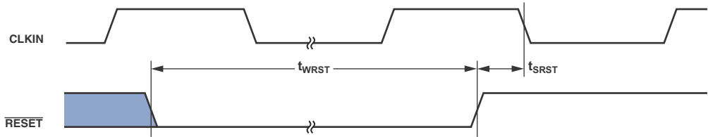
Figure 8. Reset
