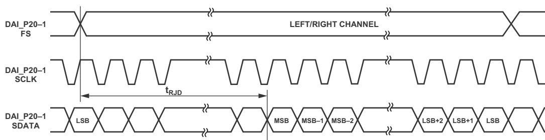
Figure 26. Right-Justified Mode
