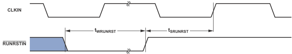
Figure 9. Running Reset
