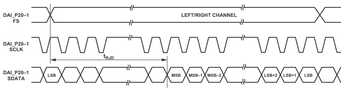
Figure 26. Right-Justified Mode
