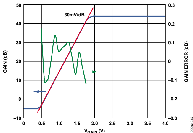
Figure 45. Linear-in-dB Gain Control Response of the X-AMP VGA Showing Consistent Slope and Low Error
