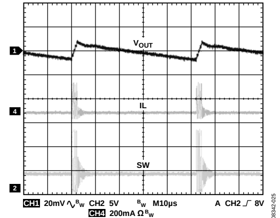
Figure 27. Steady State at Light Load, f_{SW} = 1.4 MHz , I_{OUT} = 40 mA
