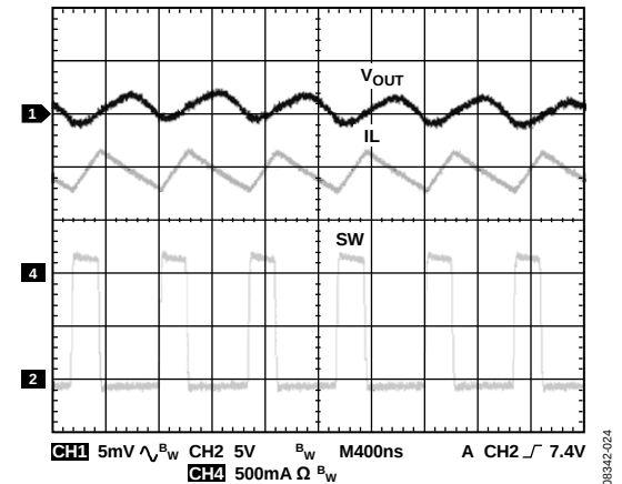
Figure 26. Steady State at Heavy Load, f_{SW} = 1.4 MHz , I_{OUT} = 1 A
