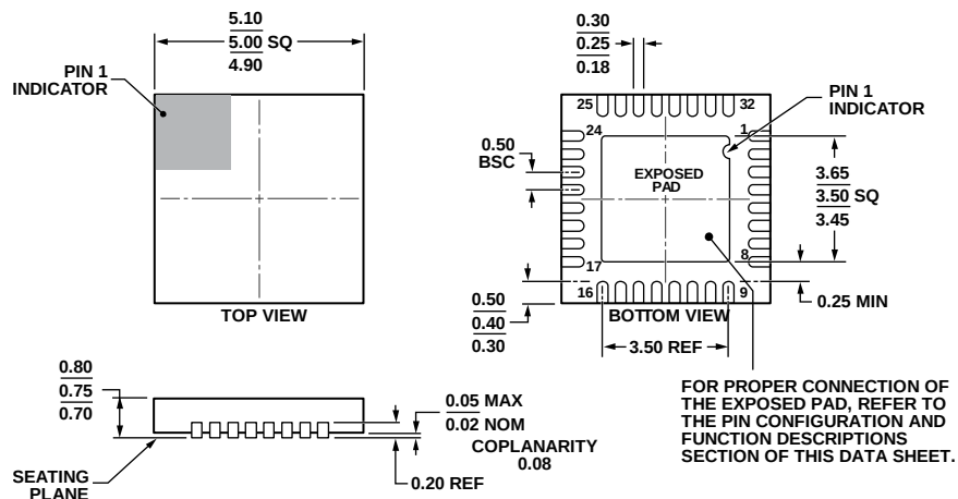
Figure 43. 32-Lead Lead Frame Chip Scale Package [LFCSP] 5 mm × 5 mm Body and 0.75 mm Package Height (CP-32-11)
