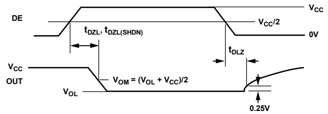
Figure 11. Driver Enable and Disable Times ( t_{DZL} , t_{DZL(SHDN)} , t_{DLZ} , t_{DLZ(SHDN)} )
