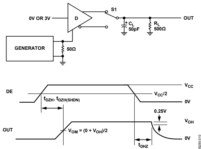
Figure 10. Driver Enable and Disable Times ( t_{DZH} , t_{DZH(SHDN)} , t_{DZL} , t_{DZL(SHDN)} )
