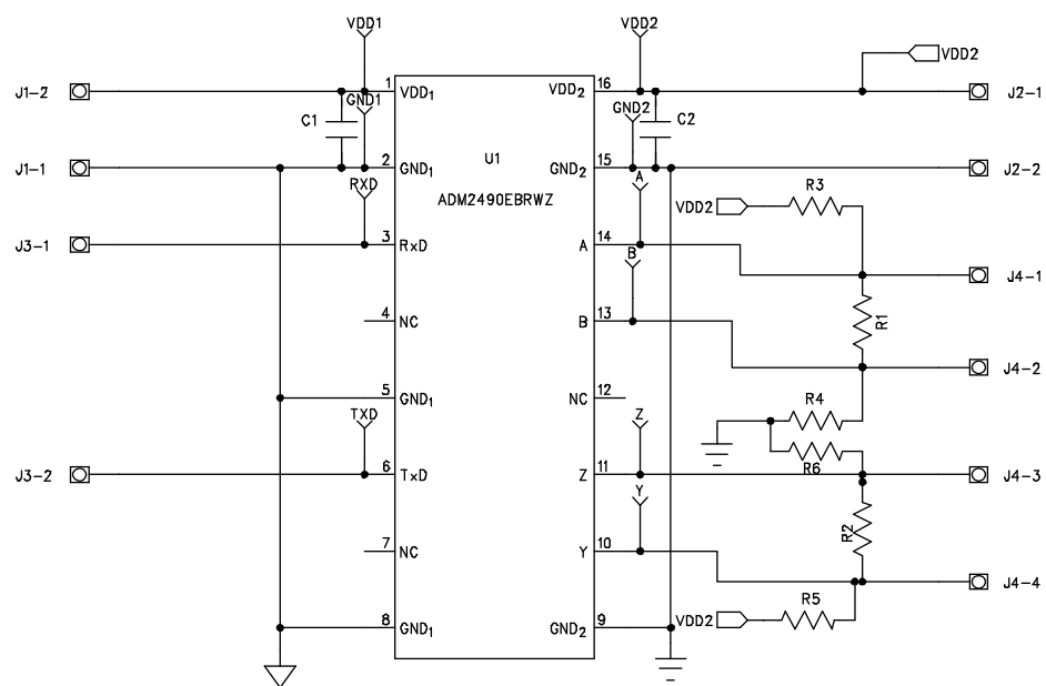
Figure 2. EVAL-ADM2490EEBZ Schematic
