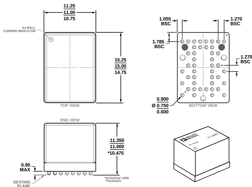
Figure 55. 44-Ball Ball Grid Array Module [BGA] (ML-44-1)
