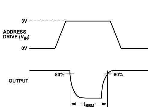
Figure 30. Break-Before-Make Delay, t_{\text{BBM}}
