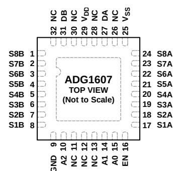
Figure 6. ADG1607 LFCSP Pin Configuration
