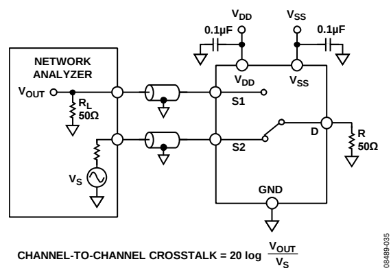
Figure 35. Channel-to-Channel Crosstalk
