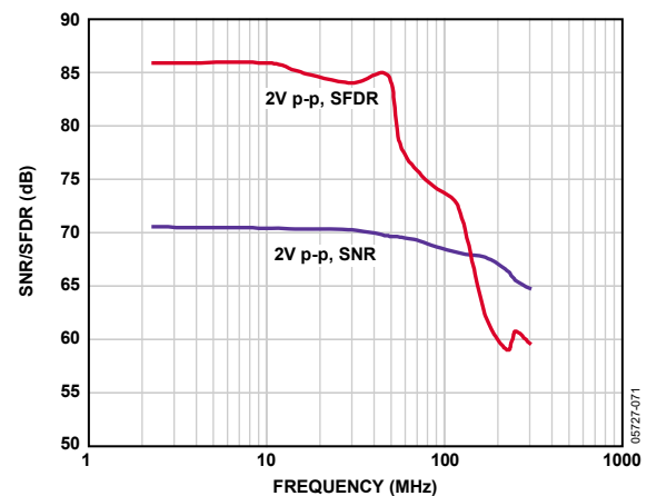
Figure 35. SNR/SFDR vs. Frequency, f_{SAMPLE} = 65 MSPS
